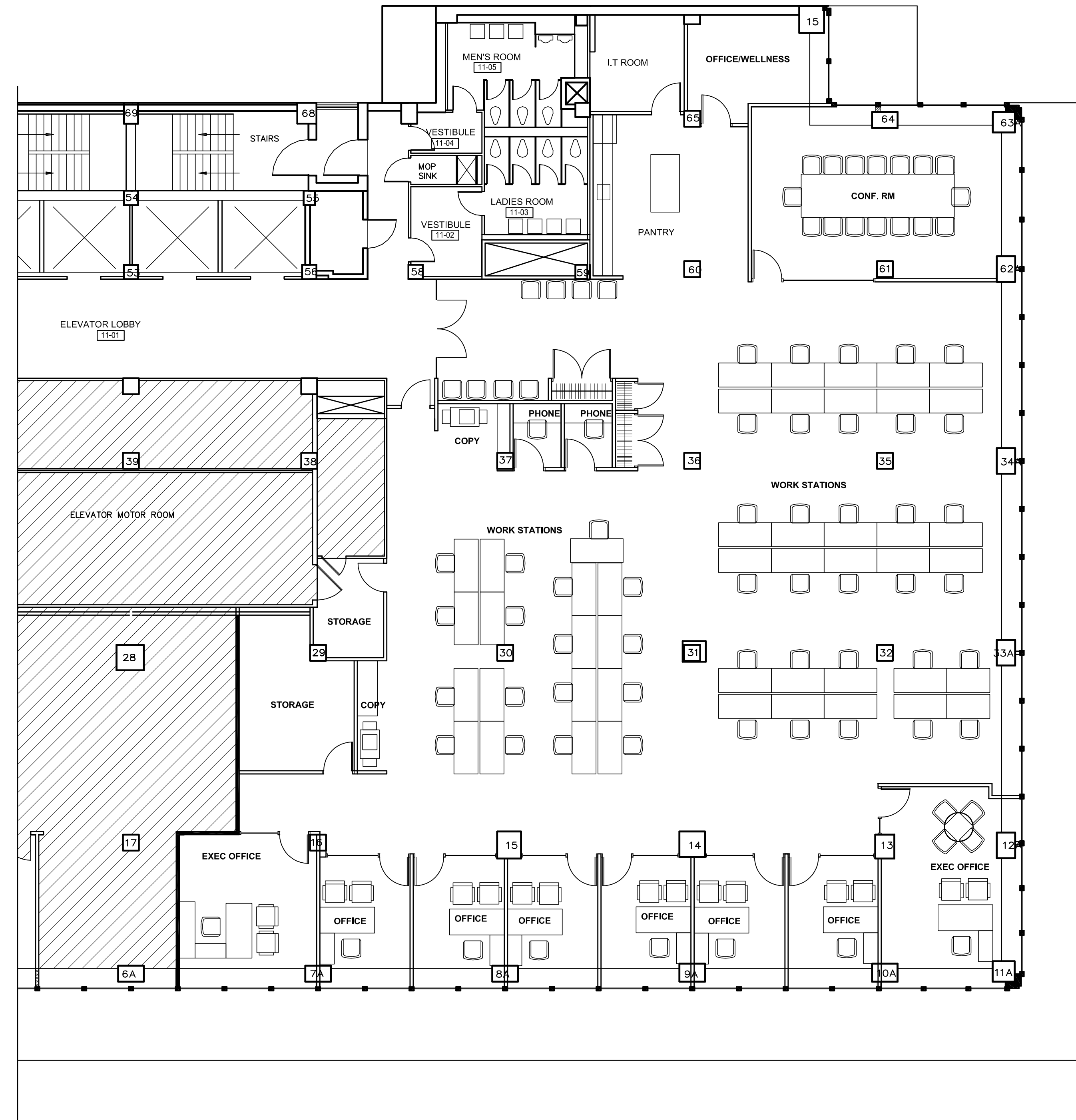
PRELIMINARY PLAN OPT 1 SCALE: 1/8"=1'-0"
