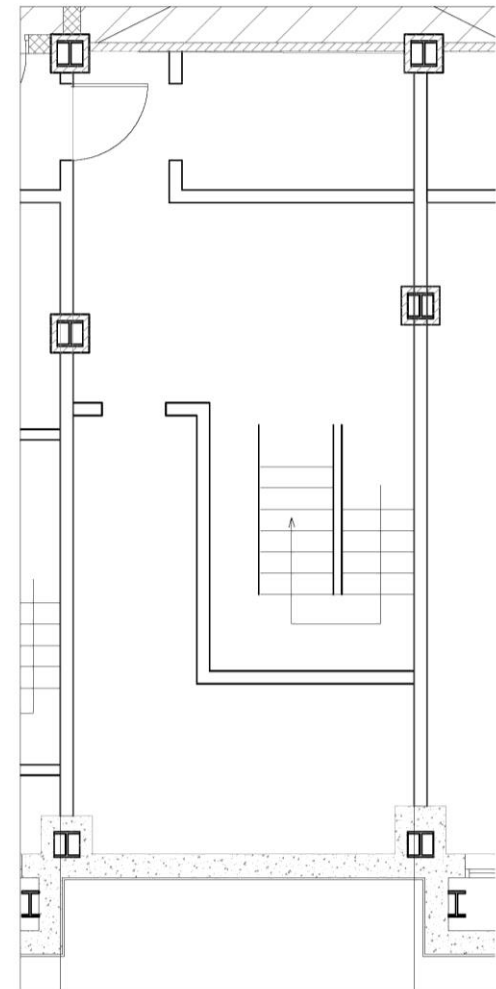
CELLAR FLOOR
