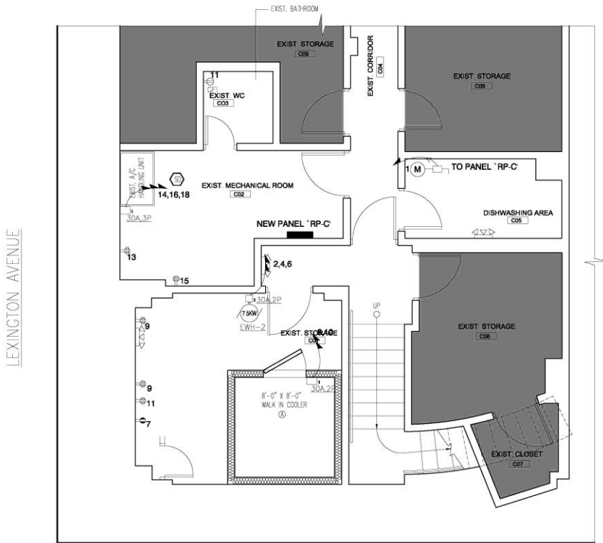
Basement: Approximately 700 SF
