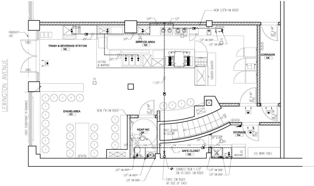
Ground Floor: Approximately 1,000 SF
