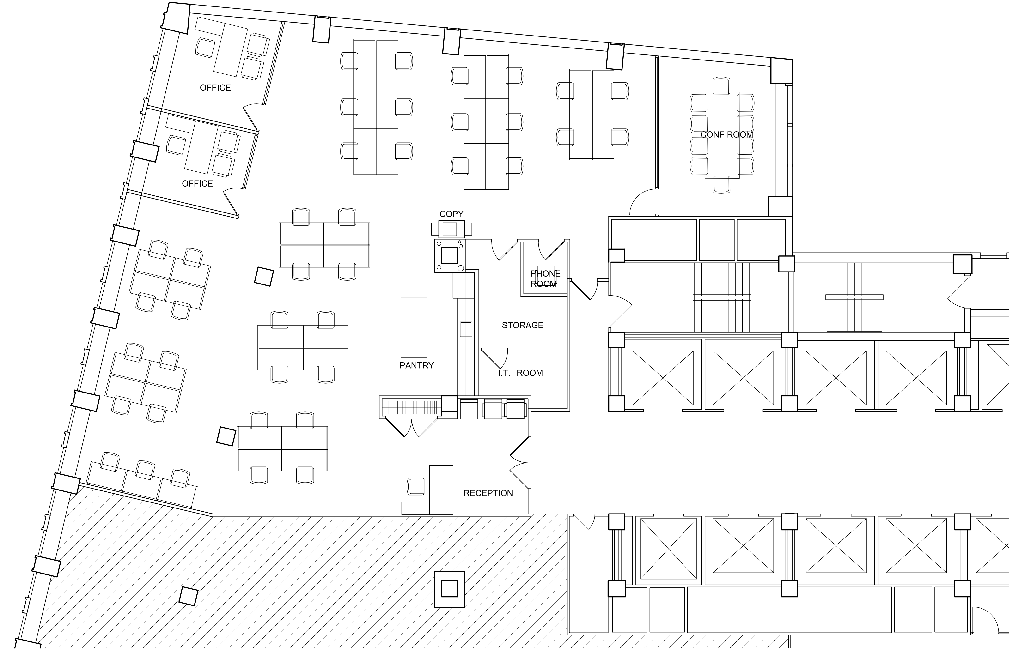
PRE-BUILT PLAN SCALE: 3/16=1'-0" PARTIAL 7TH FLOOR - 5,740 RSF
