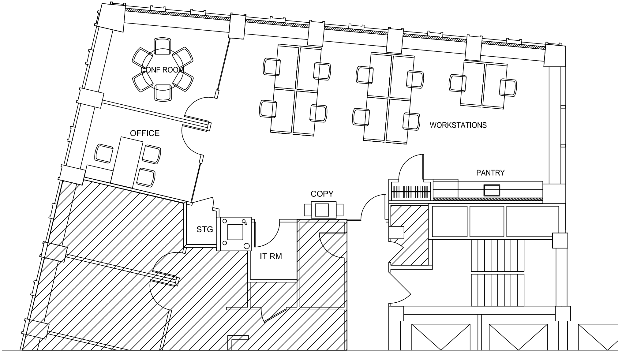
PROPOSED PRE-BUILT PLAN PARTIAL 14TH FLOOR 2,255 RSF
